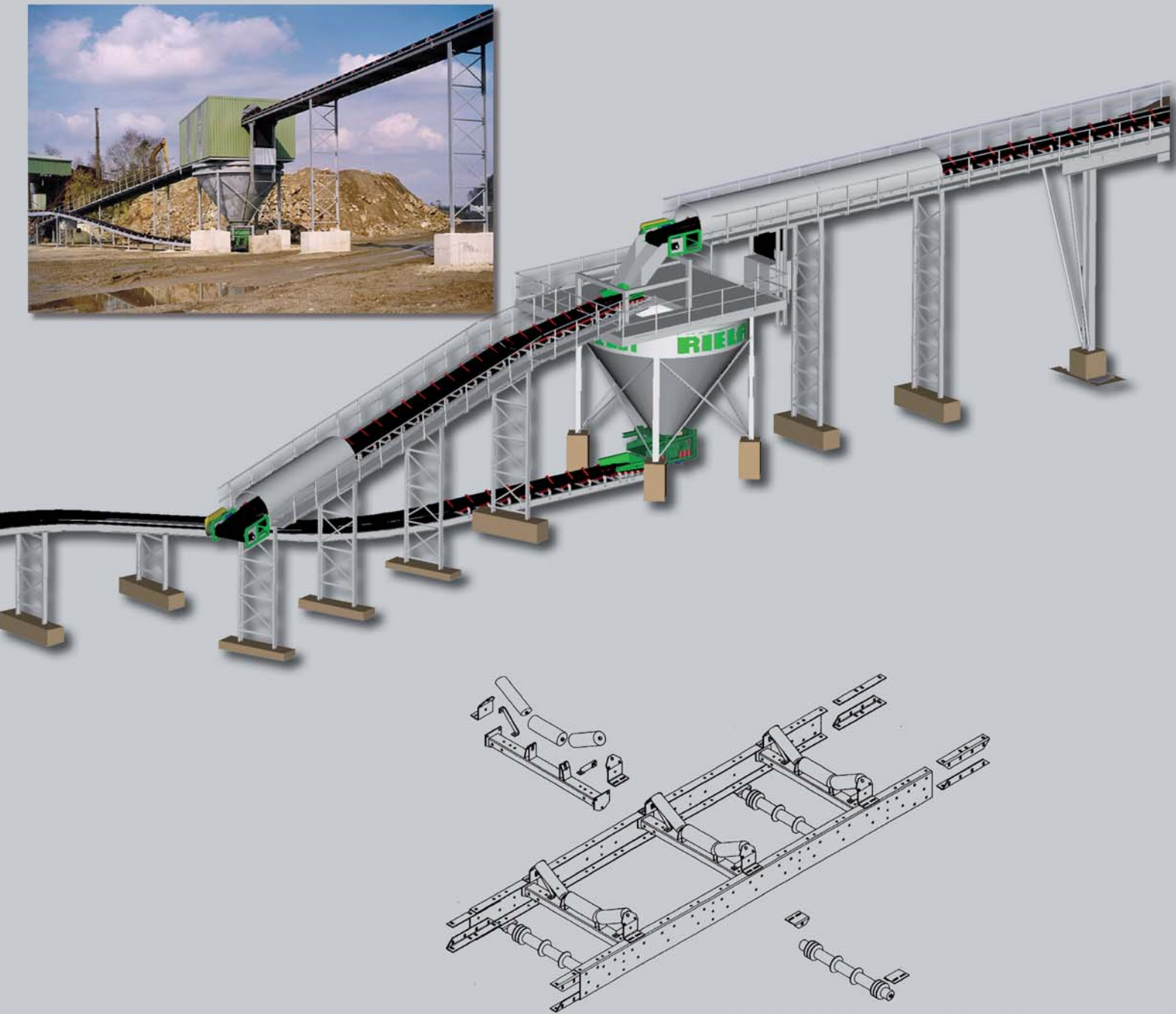
Belt conveyors as a modular construction system
